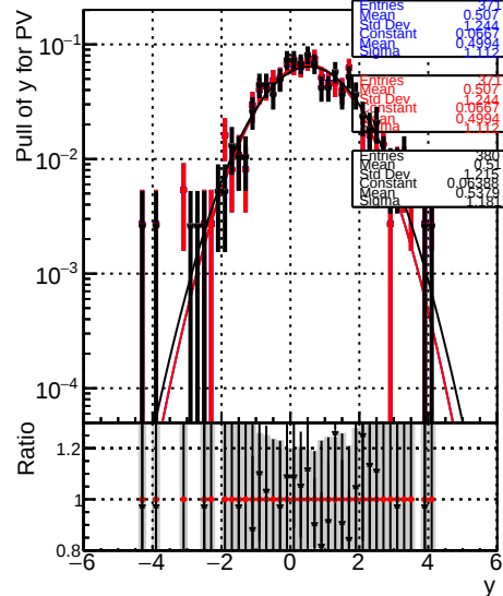
RecoPVAssoc Legend: DQM_original (blue line) DQM_original2 (red line) DQM_testMkFitExport_initialStep (black line)
