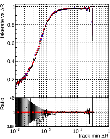
Fake rate vs \Delta R (track, jet) Legend: - DQM_original (blue line with dots) - DQM_original2 (red line with dots) - DQM_testMkFitExport_initialStep (black line with dots)
