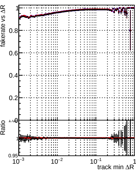
Fake rate vs \Delta R(\text{track, jet}) Legend: DQM_original (blue line with markers) DQM_original2 (red line with markers) DQM_testMkFitExport_initialStep (black line with markers)
