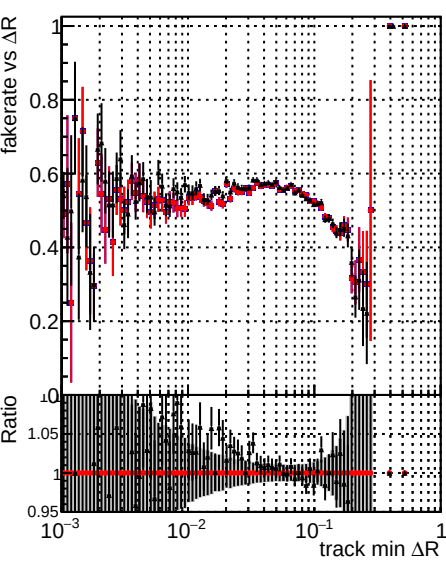
Fake rate vs \Delta R(\text{track, jet}) Legend: DQM_original (blue line with circles) DQM_original2 (red line with circles) DQM_testMkFitExport_initialStep (black line with circles)
