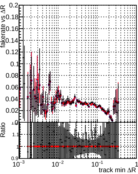
Fake rate vs \Delta R(\text{track}, \text{jet}) Legend: DQM_original (blue line with dots) DQM_original2 (red line with dots) DQM_testMkFitExport_initialStep (black line with dots)
