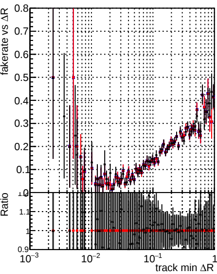
Fake rate vs ΔR(track, jet) Legend: DQM_original (blue line with dots) DQM_original2 (red line with dots) DQM_testMkFitExport_initialStep (black line with dots)
