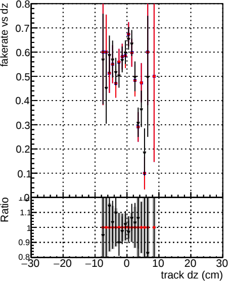
Fake rate vs dz DOM original DOM original2 DOM testMKR-rtExport initialStep
