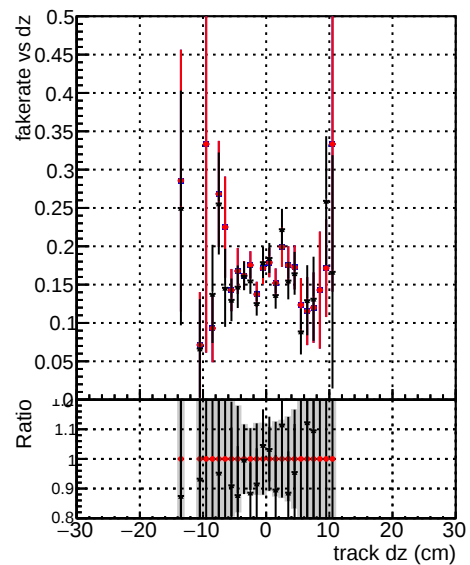
Fake rate vs dz Legend: DOM original (blue line) DOM original2 (red line) DOM testMKR-itExport initialStep (black line)
