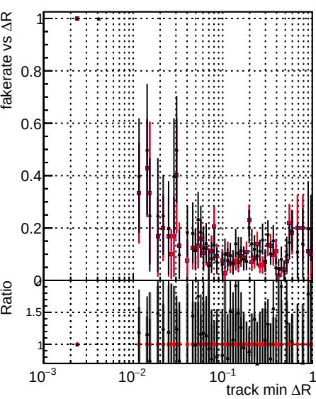
Fake rate vs \Delta R(\text{track, jet}) Legend: - \Delta R(\text{track, jet}) - \Delta R(\text{track, jet}) - \Delta R(\text{track, jet})
