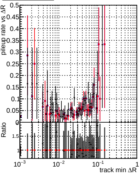
Legend: - — ● DQM_original - — ● DQM_original2 - — ● DQM_testMkFitExport_initialStep
