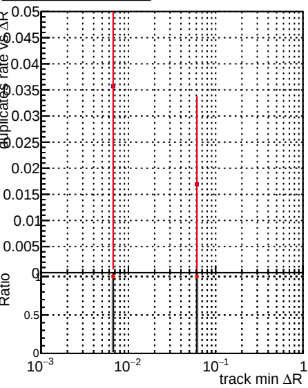
Legend: - — ● DQM_original - — ● DQM_original2 - — ● DQM_testMkFitExport_initialStep
