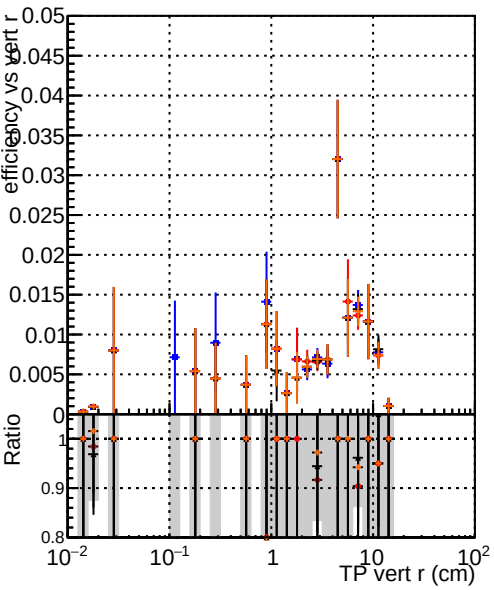
Efficiency vs TP vert r (cm) Legend: DOM_original4 DOM_testMkFit_initialStepReso DOM_testMkFitFit_initialStepReso DOM_testMkFitFit_initialStepReso_testSorting2
