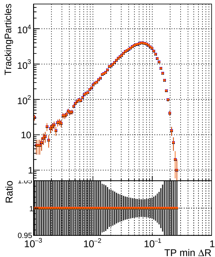
N of simulated tracks DQM_original4 DQM_testMkFit_initialStepReso DQM_testMkFitFit_initialStepReso DQM_testMkFitFit_initialStepReso_testSorting2
