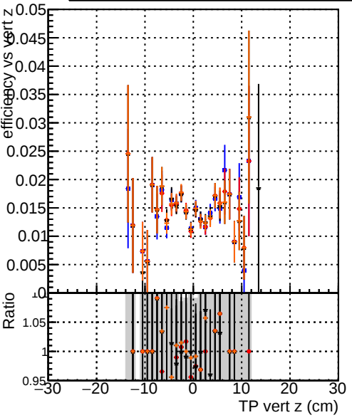
Efficiency vs vertpos Legend: DQM_original14 DQM_testMkFit_initialStepReso DQM_testMkFitFit_initialStepReso DQM_testMkFitFit_initialStepReso_testSorting2
