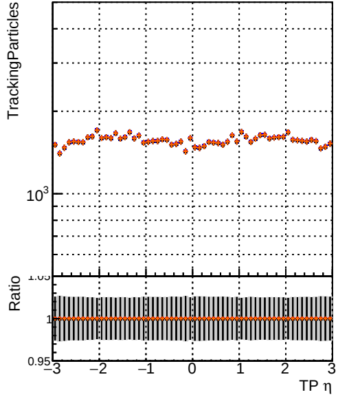
DQM_original4 DQM_testMkFit_initialStepReso DQM_testMkFitFit_initialStepReso DQM_testMkFitFit_initialStepReso_testSorting2
