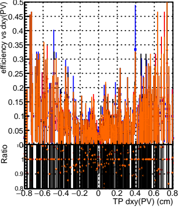
Efficiency vs Dxy(PV) legend DQM_original4 DQM_testMkFit_initialStepReso DQM_testMkFitFit_initialStepReso DQM_testMkFitFit_initialStepReso_testSorting2
