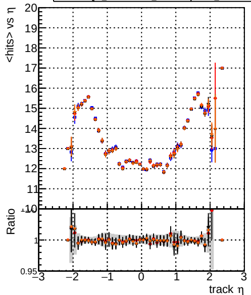
mean hits DQM_testMkFitFit_initialStepReso DQM_testMkFitFit_initialStepReso_testSorting2 DQM_testMkFitFit_initialStepReso DQM_testMkFitFit_initialStepReso
