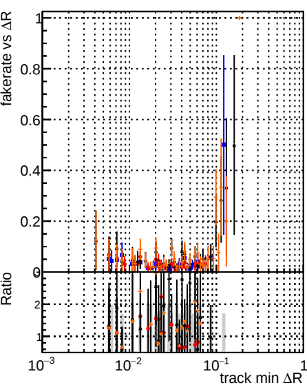
Fake rate vs \Delta R(\text{track, jet}) Legend: DOM original4 DOM testIMKFit initialStepReso DOM testIMKFit initialStepReso testSorting2
