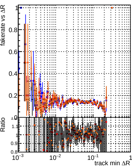
Fake rate vs \Delta R(\text{track, jet}) DQM original4 testIMKFit initialStepReso testIMKFit initialStepReso testSorting2
