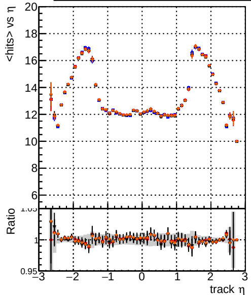
DQM_original4 DQM_testMkFit_fit_initialStepReso DQM_testMkFitFit_initialStepReso DQM_testMkFitFit_initialStepReso_testSorting2 mean hit
