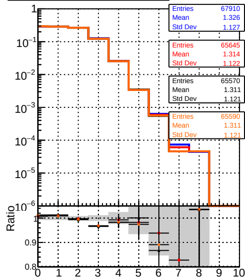
DQM_original4 DQM_testMkFit_fit_initialStepReso DQM_testMkFitFit_initialStepReso DQM_testMkFitFit_initialStepReso_testSorting2 mean hit
