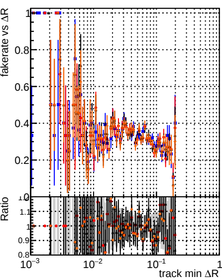
Fake rate vs \Delta R (track, jet) for various methods: DOM original, testIMKFit, testIMKFit_initialStepReso, testIMKFit_initialStepReso_testSorting2
