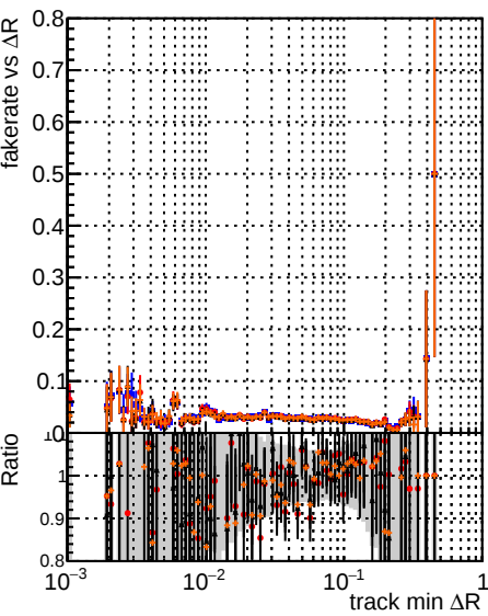
Fake rate vs \Delta R(\text{track}, \text{jet}) DQM original4 testIMKFit_initialStepReso testIMKFit_initialStepReso testIMKFit_testSorting2
