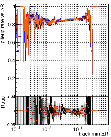
Legend: DOM original, DOM test, DOM testIMKFit, DOM testIMKFit initialStepReso, DOM testIMKFit initialStepReso testSorting2
