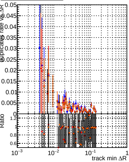
Legend: DOM original, DOM test, DOM testIMKFit, DOM testIMKFit initialStepReso, DOM testIMKFit initialStepReso testSorting2
