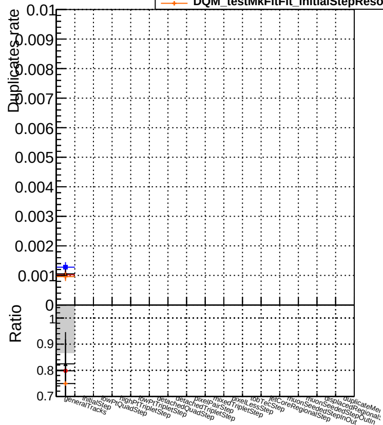
Duplicates rate vs \epsilon ● DQM_testMkFit_initialStepReso ▲ DQM_testMkFitFit_initialStepReso + DQM_testMkFitFit_initialStepReso_testSorting2
