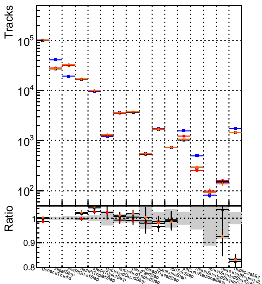
■ DQM_original4 ● DQM_testMkFit_initialStepReso ★ DQM_testMkFitFit_initialStepReso ▲ DQM_testMkFitFit_initialStepReso_testSorting2
