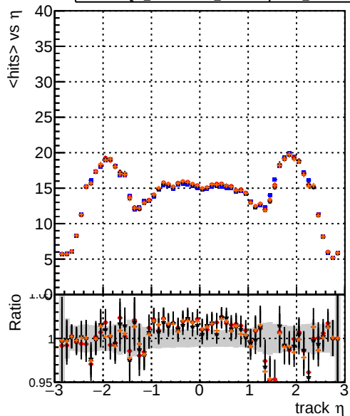
DQM_testMkFit_initialStepReso DQM_testMkFitFit_initialStepReso DQM_testMkFitFit_initialStepReso_testSorting2 mean hits
