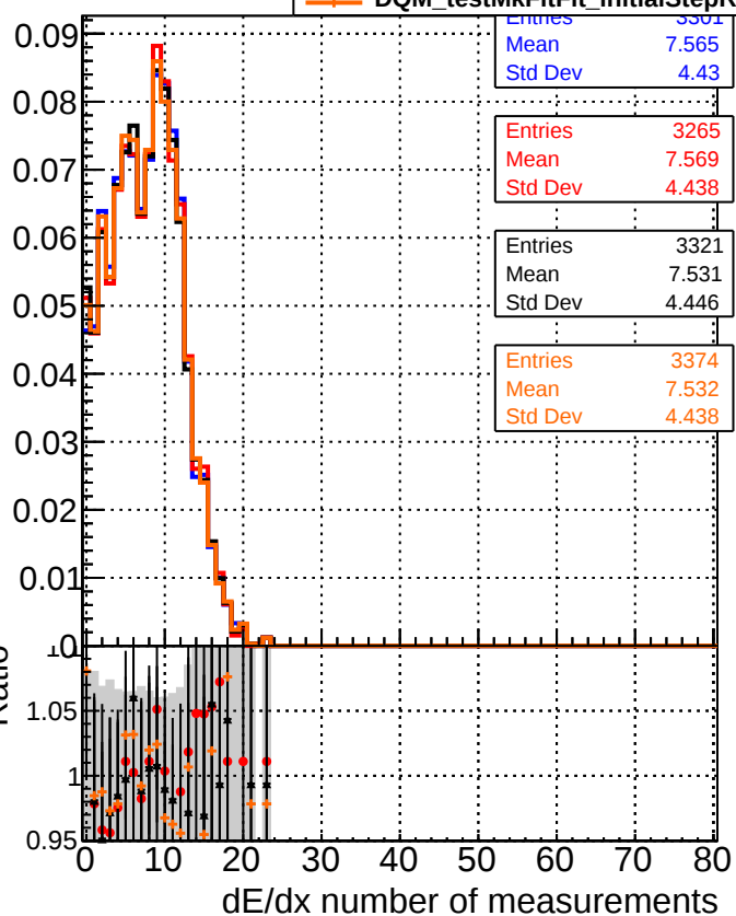
—●— DQM_original4 —●— DQM_testMkFit_initialStepReso —●— DQM_testMkFitFit_initialStepReso —●— DQM_testMkFitFit_initialStepReso_testSorting2
