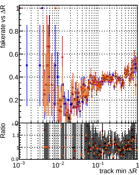
Fake rate vs \Delta R(\text{track, jet}) DOM original DOM test DOM testIMKFit initialStepReso DOM testIMKFit initialStepReso testSorting2
