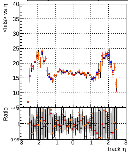
mean hits vs \eta Legend: DQM_original4 (blue line), DQM_testMkFit_fit_initialStepReso (red line), DQM_testMkFitFit_initialStepReso (black line), DQM_testMkFitFit_initialStepReso_testSorting2 (orange line)
