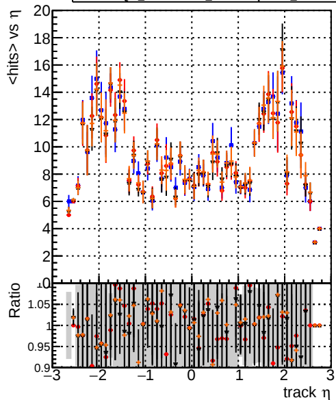
DQM_original4 DQM_testMkFit_fit_initialStepReso DQM_testMkFitFit_initialStepReso DQM_testMkFitFit_initialStepReso_testSorting2 mean hit
