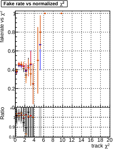
Fake rate vs. DOM original4 DOM testMRFFit-InitialStepReso DOM testMRFFit-InitialStepReso testSorting2
