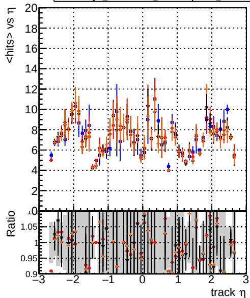
DQM_original14 DQM_testMkFitFit_initialStepReso DQM_testMkFitFit_initialStepReso DQM_testMkFitFit_initialStepReso_testSorting2
