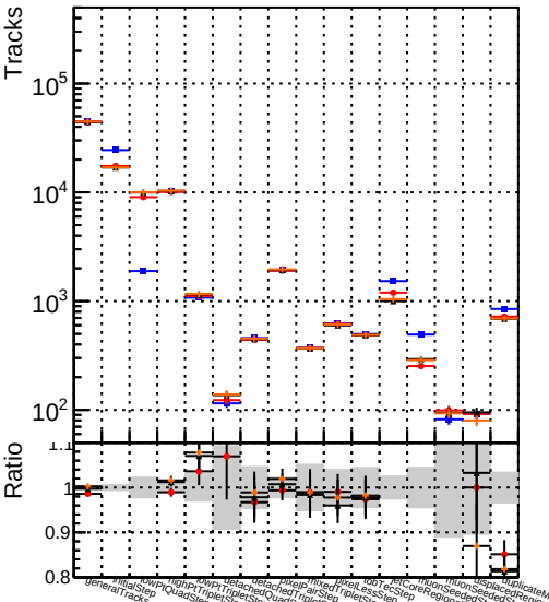
Number DQM_original4 DQM_testMkFit_initialStepReso DQM_testMkFitFit_initialStepReso DQM_testMkFitFit_initialStepReso_testSorting2
