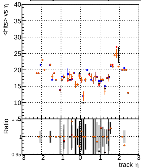
mean hit DQM_original4 DQM_testMkFit_initialStepReso DQM_testMkFitFit_initialStepReso DQM_testMkFitFit_initialStepReso_testSorting2
