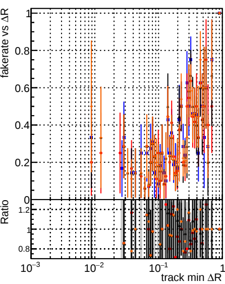
Fake rate vs \Delta R(\text{track, jet}) DOM original DOM test DOM IMKFit initialStepReso DOM IMKFit initialStepReso testSorting2
