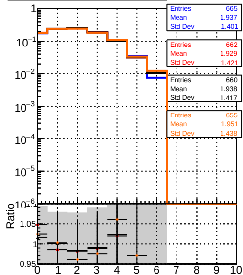
mean hit — DQM_original4 — DQM_testMkFitFit_initialStepReso — DQM_testMkFitFit_initialStepReso — DQM_testMkFitFit_initialStepReso_testSorting2
