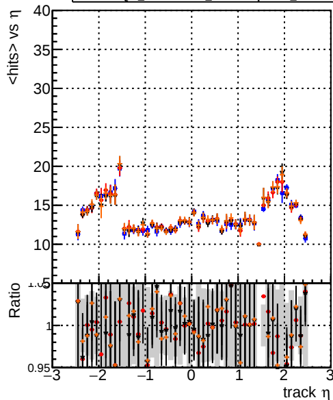
mean hit DQM_original4 DQM_testMkFit_initialStepReso DQM_testMkFitFit_initialStepReso DQM_testMkFitFit_initialStepReso_testSorting2
