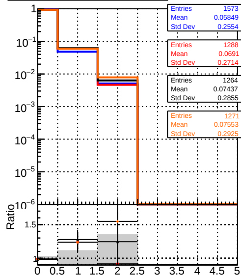
mean hit DQM_original4 DQM_testMkFit_initialStepReso DQM_testMkFitFit_initialStepReso DQM_testMkFitFit_initialStepReso_testSorting2
