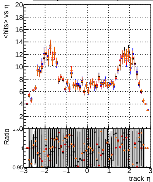
mean hit DQM_original4 DQM_testMkFit_fit_initialStepReso DQM_testMkFitFit_initialStepReso DQM_testMkFitFit_initialStepReso_testSorting2
