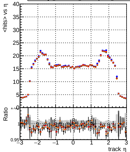
mean hit DQM_original DQM_testMkFit_initialStepReso DQM_testMkFitFit_initialStepReso DQM_testMkFitFit_initialStepReso_testSorting2
