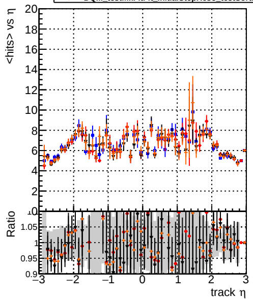
mean hits vs \eta Legend: DQM_original4 (blue line), DQM_testMkFit_initialStepReso (red line with error bars), DQM_testMkFitFit_initialStepReso (black line with error bars), DQM_testMkFitFit_initialStepReso_testSorting2 (orange line with error bars)
