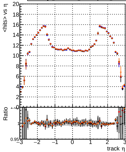
Legend for mean hits vs \eta : Blue line: DQM_original4 Red line: DQM_testMkFit_initialStepReso Black line: DQM_testMkFitFit_initialStepReso Orange line: DQM_testMkFitFit_initialStepReso_testSorting2
