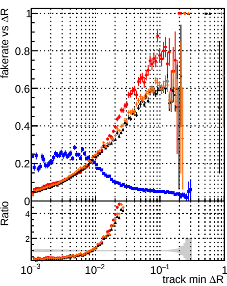
Fake rate vs \Delta R(\text{track, jet}) DQM original4 testIMKFit_initialStepReso testIMKFit_initialStepReso testIMKFit_initialStepReso testSorting2
