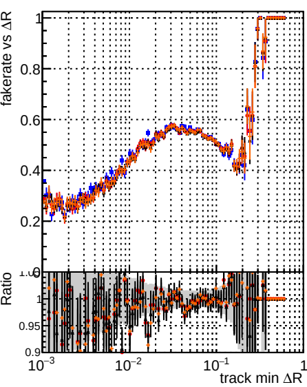
Fake rate vs \Delta R(\text{track, jet}) Legend: original (blue), testIMKFit (red), testIMKFit initialStepReso (black), testIMKFit initialStepReso testSorting2 (orange).
