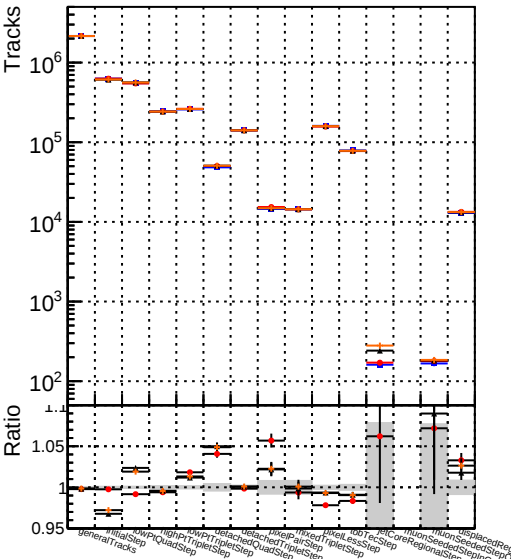
Number — DQM original — DQM testMkFit_initialStepReso — DQM testMkFitFit_initialStepReso — DQM testMkFitFit_initialStepReso testSorting2
