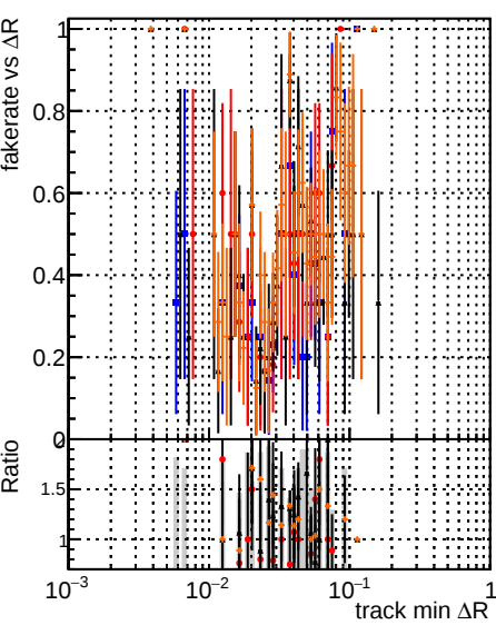
Fake rate vs \Delta R(\text{track, jet}) Legend: DOM original (blue) DOM test (red) DOM testIMKFit (black) DOM testIMKFit initialStepReso (orange) testIMKFit initialStepReso testSorting2 (green)
