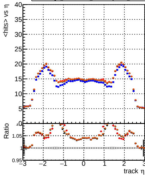
mean hit DQM_original DQM_testMkFit_initialStepReso DQM_testMkFitFit_initialStepReso DQM_testMkFitFit_initialStepReso_testSorting2
