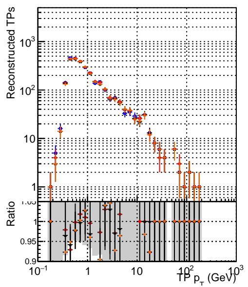
● DQM_original14 ● DQM_testMkFit_initialStepReso ● DQM_testMkFitFit_initialStepReso ● DQM_testMkFitFit_initialStepReso_testSorting2
