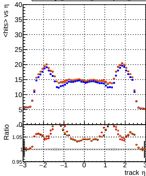
mean hits DQM_original DQM_testMkFit_initialStepReso DQM_testMkFitFit_initialStepReso DQM_testMkFitFit_initialStepReso_testSorting2
