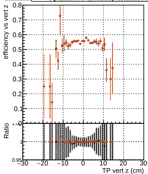
Efficiency vs vert z —●— DQM_original4 —●— DQM_testMkFit_initialStepReso —●— DQM_testMkFitFit_initialStepReso —●— DQM_testMkFitFit_initialStepReso_testSorting2
