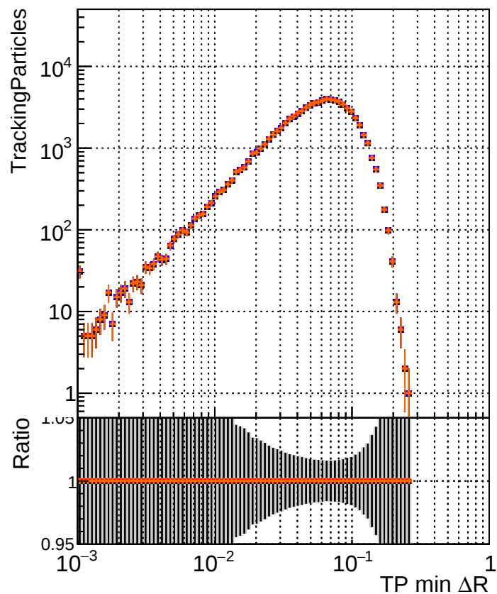
N of simulated tracks DQM_original4 DQM_testMkFit_initialStepReso DQM_testMkFitFit_initialStepReso DQM_testMkFitFit_initialStepReso_testSorting
